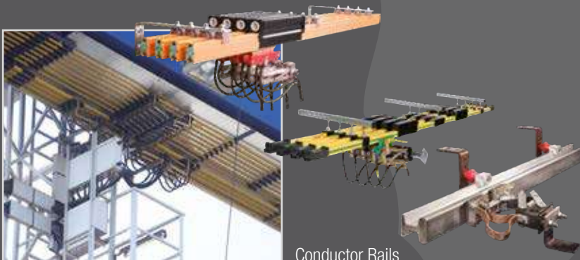
Conductor Rails
