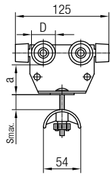
Cable Trolley
