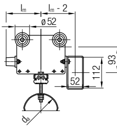
Towing Trolley
