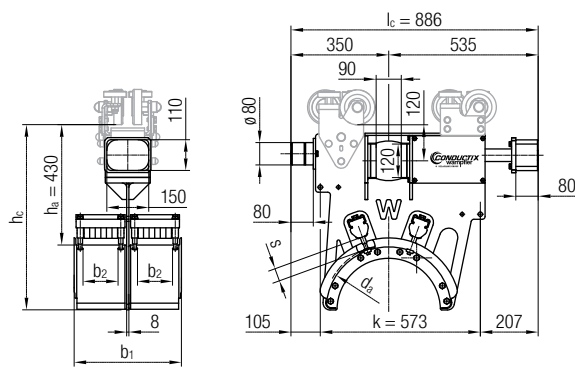
Towing trolley for catenary trolley
