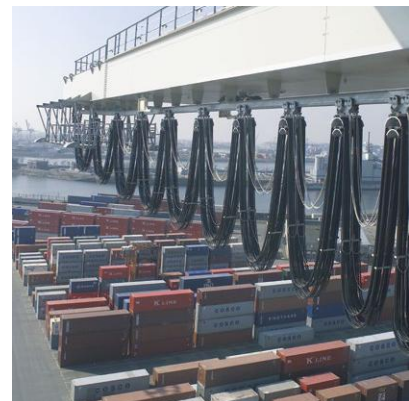
Supply of the crab on a fast travelling STS-container crane
