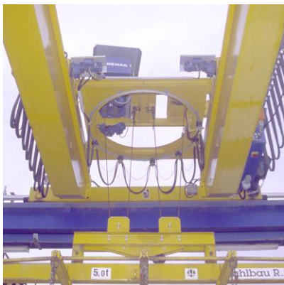
Supply of the turning-crab on an EOT-crane
