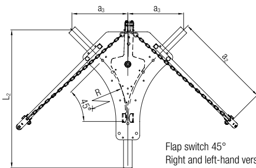
Flap switch 45° Right-hand version Chain-hoist operated
