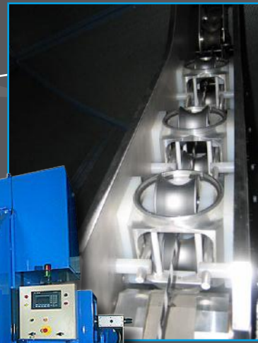
Rollertwist strander: a real Unilay
