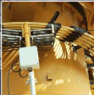
Conductor Rails on a boom stacker
